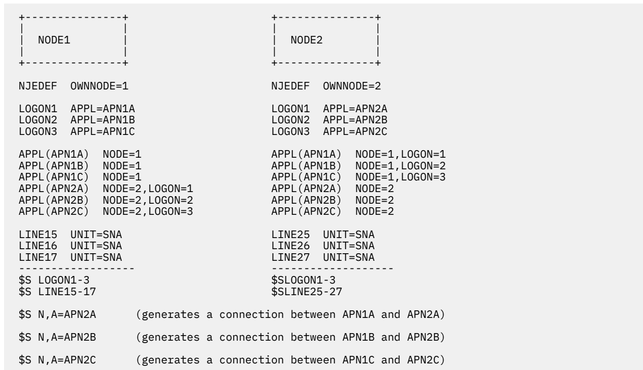
Figure 72. Parallel SNA NJE sessions between two nodes
