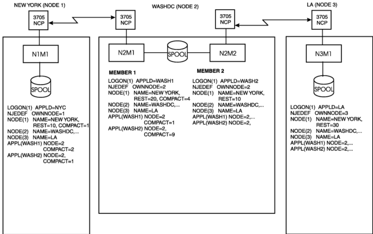
Figure 92. Multi-Access Spool Configuration (SNA)
