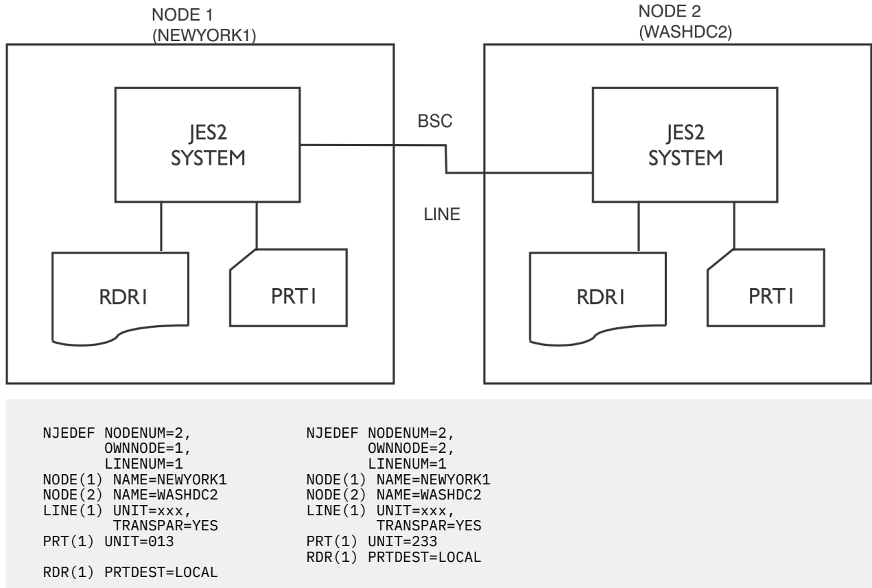
Figure 69. Minimum NJE Configuration (BSC only)
