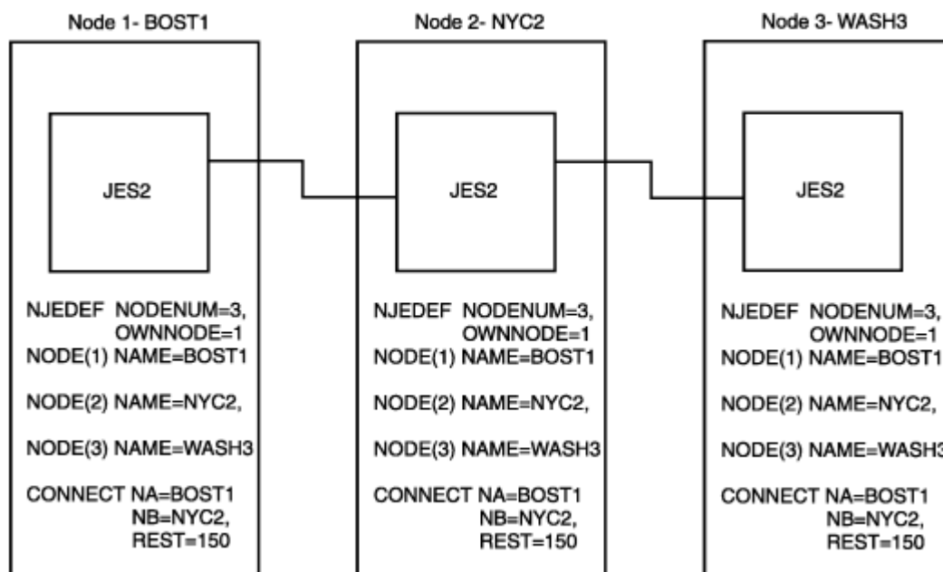
Figure 83. Static connections
